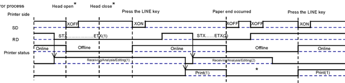
(2) Error process
